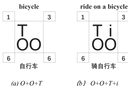
Figure 1. Cosmic language:
