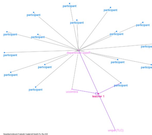
Figure 2. “Hierarchical-Bottleneck”.
